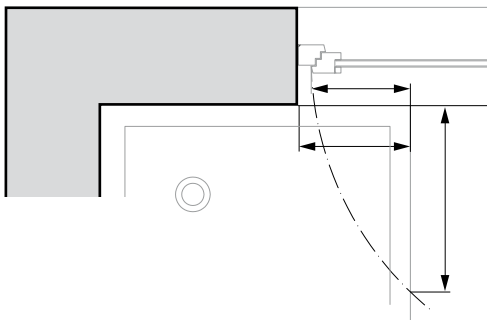
Detail Fenster
